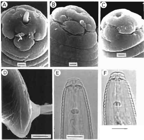
Fig. 5. SEM (A-D) and LM (E-F) photographs of males of Meloidogyne fallax n. sp. (A, B, D, E) and M. chitwoodi (C, F). A : Cephalic region (face view); B, C : Cephalic region (lateral view); D : Tail (lateral view); E, F : Cephalic region (lateral view). (Scale bars : A, B, C = 1 \mu m; D = 5 \mu m; E, F = 10 \mu m).
