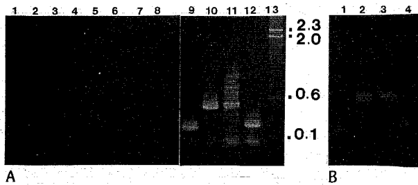
FIG. 2. (A) Successful amplification of target DNA is dependent on the reaction buffer. Lanes: 1 to 4, buffer I; 5 to 8, buffer II; 9 to 12, buffer III. Primer pair 2-3 was used for samples 1, 5, and 9; primer pair 4-5 was used for samples 2, 6, and 10; primer pair 6-7 was used for samples 3, 7, and 11; and primer pair 1-5 was used for samples 4, 8, and 12. The annealing temperature was 55°C. (B) As for panel A, lanes 9 to 12, except that the annealing temperature was 60°C. The sizes (in kilobases) of lambda HindIII standards (lane 13) are given between the panels. The template DNA was 50 ng of EcoRI-digested pathotype A (XC62) DNA for all reactions. Arrowheads in the right margin denote the expected positions of specific amplification products.
