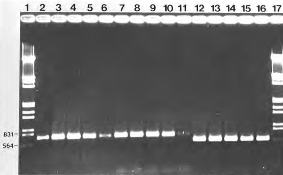
Fig. 3. Agarose gel electrophoresis of the products of the polymerase chain reaction amplification of DNA from various strains of Xylella fastidiosa with three primer sets. Lanes 2–6, primers RST29/RST30; lanes 7–11, primers RST31/RST33; and lanes 12–16, primers RST32/RST33. Target DNA (100 ng) sources: lanes 2, 7, and 12, Pierce's disease strain PCE-RR (ATCC 35879); lanes 3, 8, and 13, plum leaf scald strain PLM-G83 (ATCC 35871); lanes 4, 9, and 14, citrus variegated chlorosis strain IAPAR 10437; lanes 5, 10, and 15, oak leaf scorch strain OAK (ATCC 35874); and lanes 6, 11, and 16, sycamore leaf scorch strain SYC86-1. Lanes 1 and 17 contain 0.5 \mu g of EcoRI + HindIII -digested \lambda DNA. Molecular weights of markers are given in base pairs.
